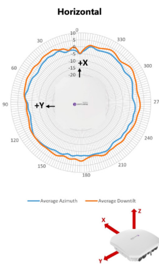
Azimuth plane (top view) – 6.50GHz
