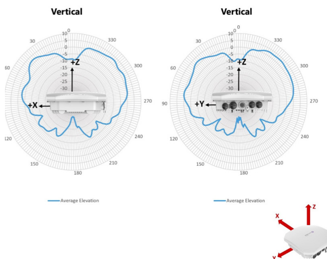
Elevation plane (side view) – 6.50GHz
